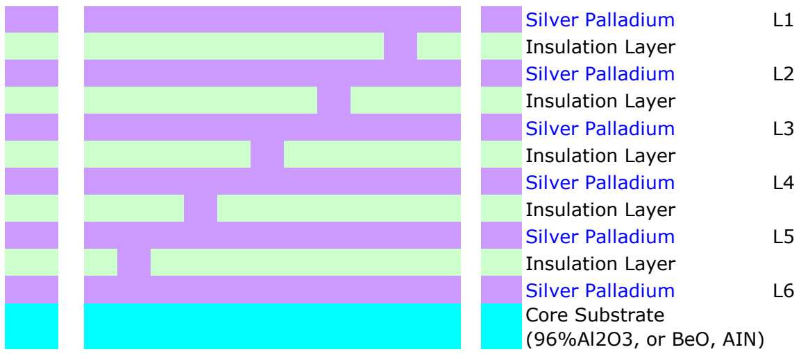
6L Ceramic PCB
