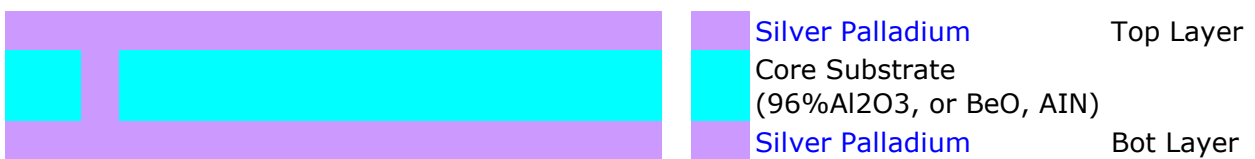
Double Sided Ceramic PCB
