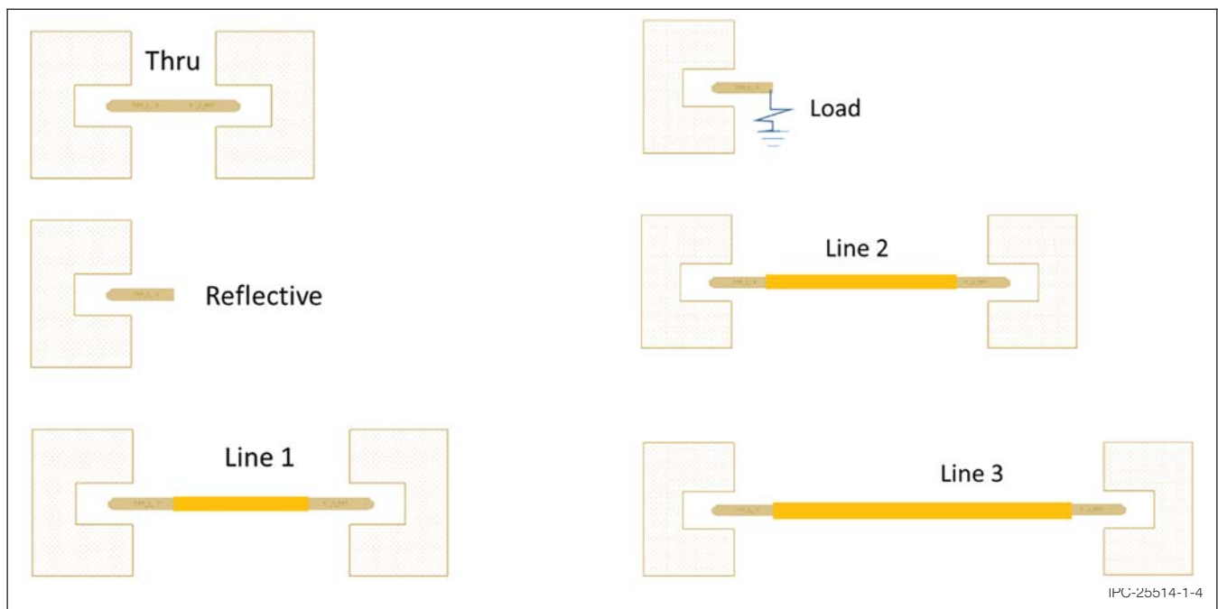
Figure 1-4 Calibration Structures (with probing footprint) for a TRL Calibration Example
