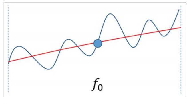
Figure 5-5 Deviation of the Raw Data from the Fitted Curve at a Single Frequency Point can be Misleading
