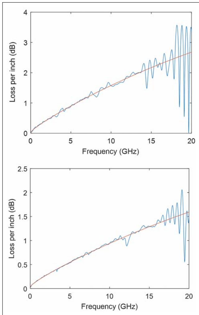
Figure 5-4 Examples of an Alternative Insertion Loss Fitting using Eq. 6
