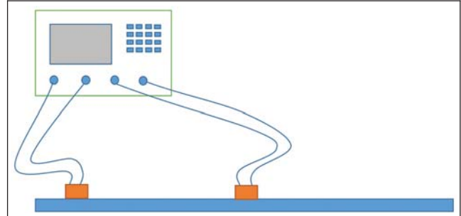
Figure 4-1 Typical VNA Measurement Setup
