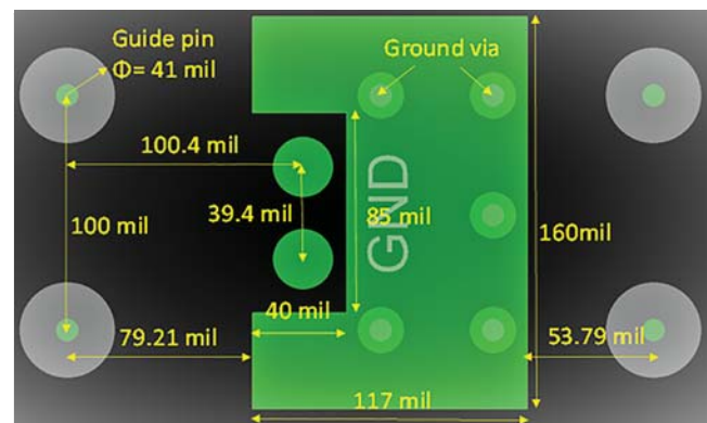
Figure 3-1 Example of a Probe Launch Footprint for Differential Signal Probing (both footprint and dimensions are shown for informative purposes only)
