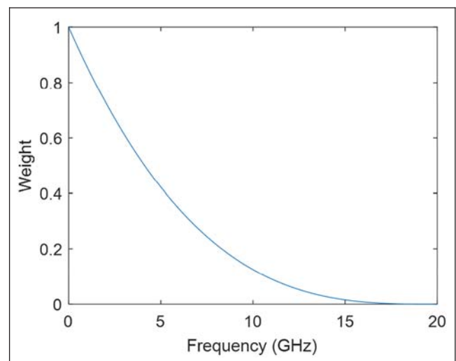
Figure 5-3 The Suggested Weight Function for Insertion Loss Curve Fitting
