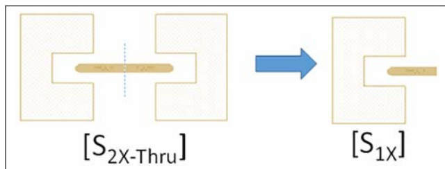
Figure 1-5 S parameter of Test Fixture is Calculated from S Parameter of 2X-Thru
