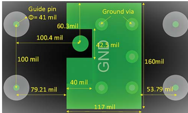
Figure 3-2 Example of a Probe Launch Footprint for Single-ended Signal Probing (both footprint and dimensions are shown for informative purposes only)
