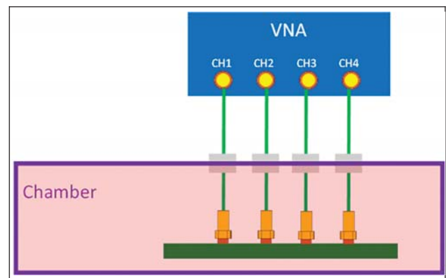
Figure 5-6 Temperature Experiment Setup
