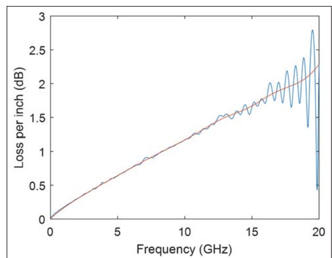
Figure 5-1 An Iterative Moving Average Applied to a Typical Insertion Loss Curve
