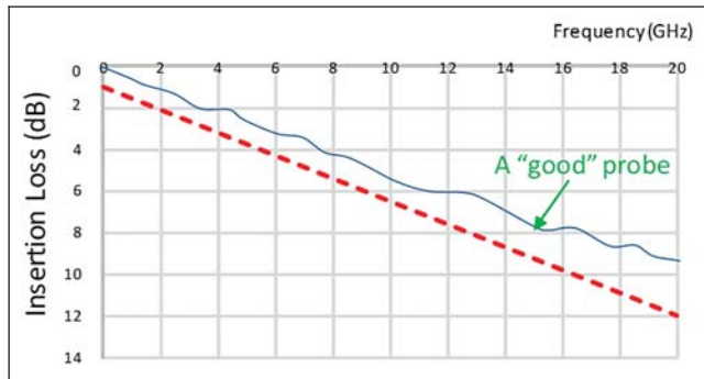
Figure 4-3 Insertion Loss Requirement for the Probe Quality Test Setup in Figure 4-2
