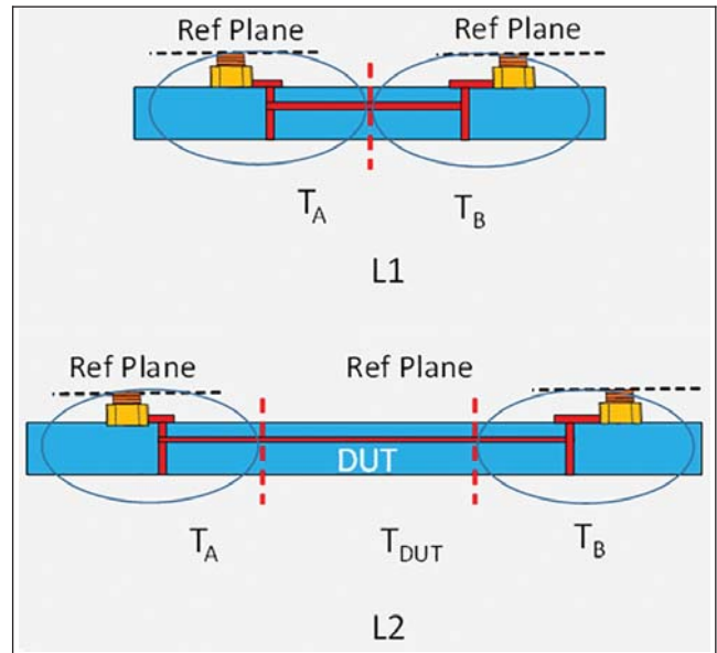
Figure 1-3 Two-line Structure for Eigenvalue-based Method
